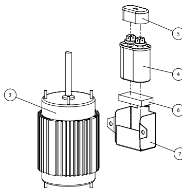
Figure 3.2a: #110002-010 Parts Diagram
