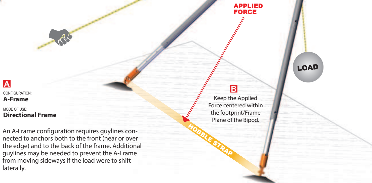
TOP VIEW
