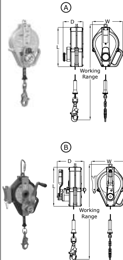
Figure 1 – Ultra-Lok™ Self-Retracting Lifelines with Integral Rescue (SLR-R)
