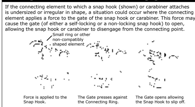
Figure 4 – Unintentional Disengagement
