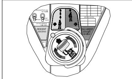
Diagram 5 – RSQ Knob
