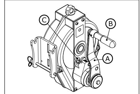
Diagram 6 – Hand Crank
