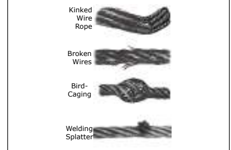
Diagram 3 – Lifeline
