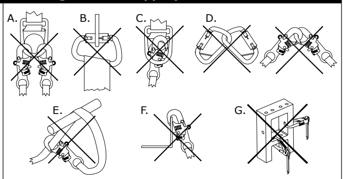
Figure 5 – Inappropriate Connections
