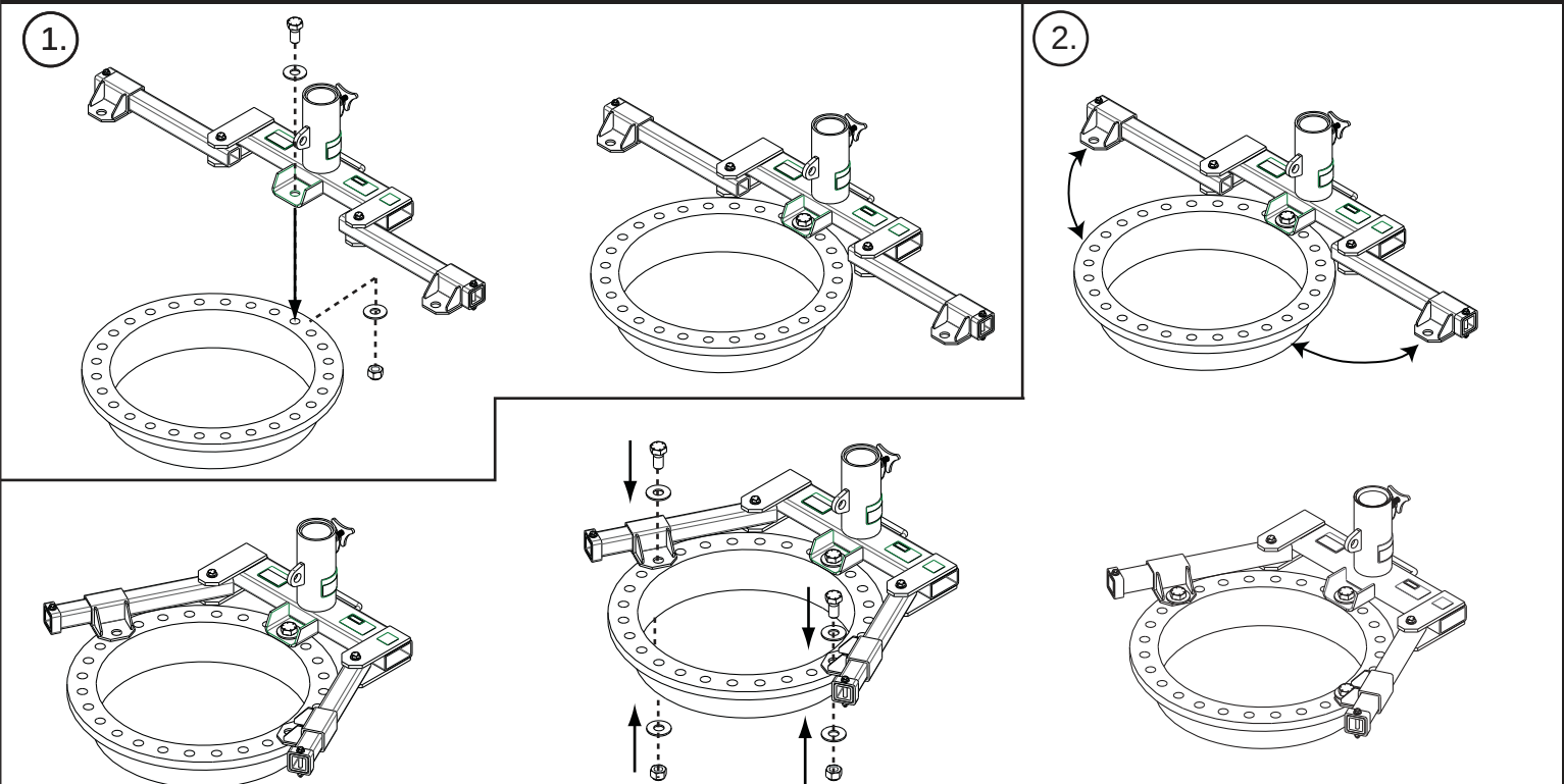
Figure 2 - INSTALLATION
