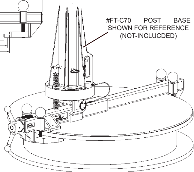
ISOMETRIC VIEW (CLAMP SHOWN ON 34" FLANGE MANWAY WITH #FT-C70 TOWER)
